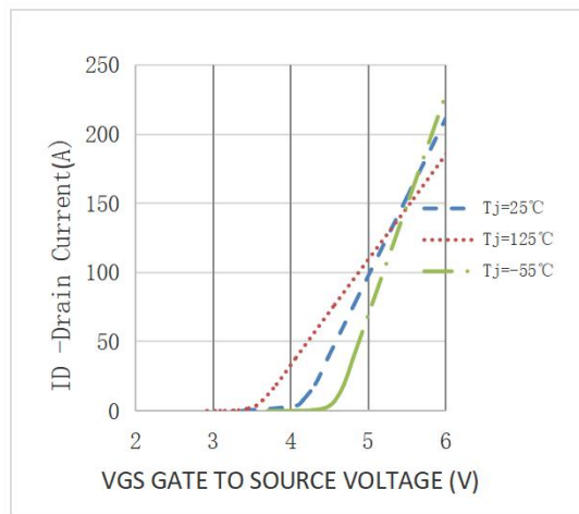
Figure 10. Transfer Characteristics
