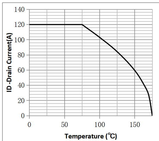
Fig.12 ID vs. Case Temperature ③
